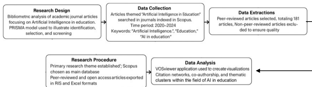
Figure 2. Research Flowchart
